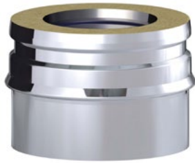
Colector hollín para chimenea DINAK DW PELLETS inox. AISI316L/304 Ø80/140mm
