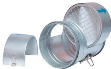
Recambio filtro intercalable "NECK" MCM G4 Ø300mm MERCATUB
