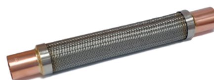
Antivibrador Flexible 2-5/8" Acero Inoxidable
