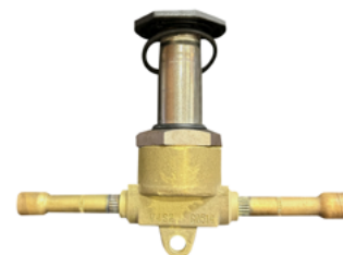
Valvula solenoide PARKER V8S4 1/2" soldar
